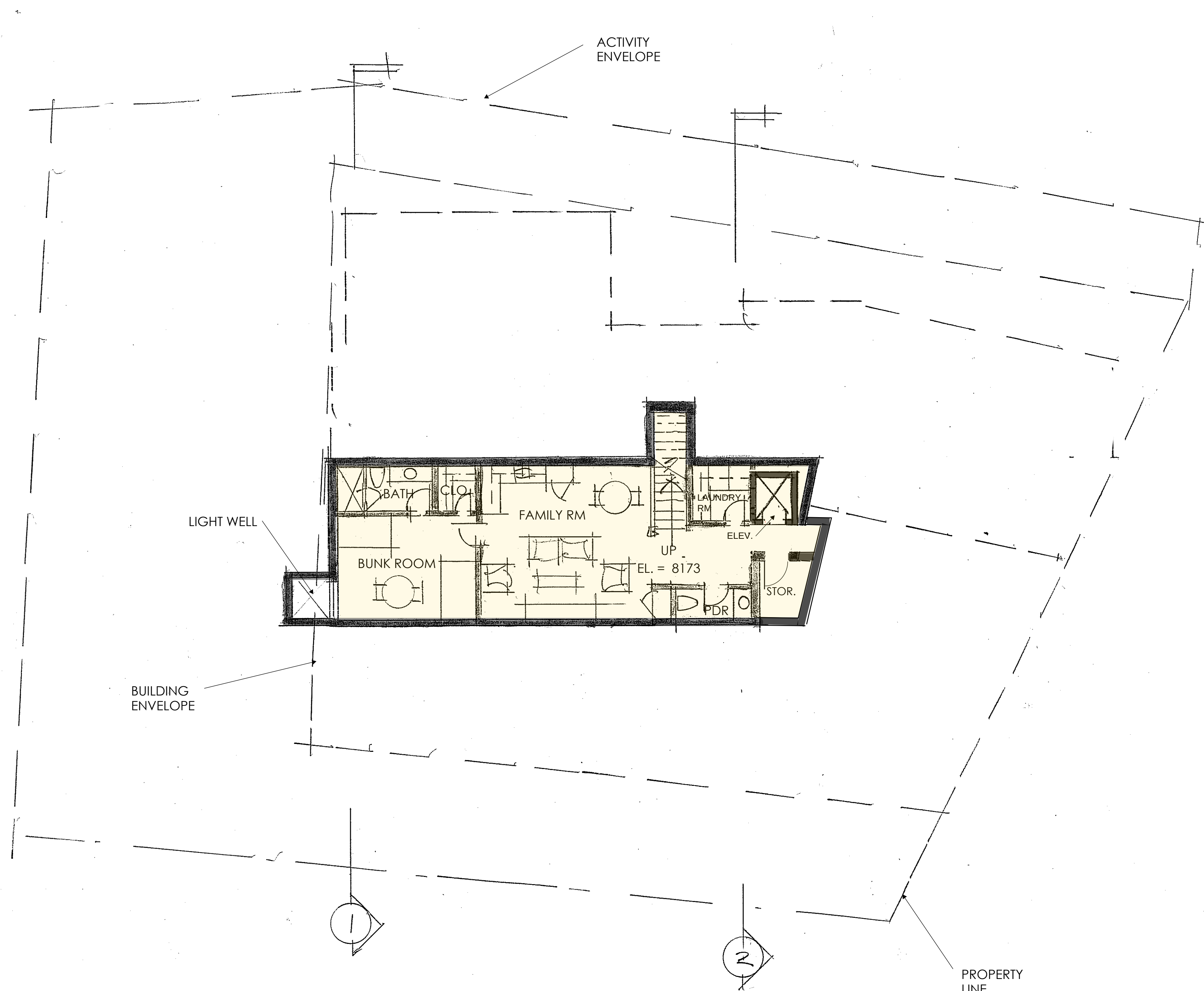
BASEMENT PLAN
